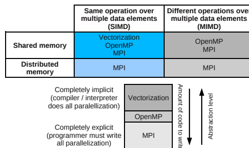
Figure 1: Comparison of three parallelization paradigms. Top: With respect to the number of different simultaneous operations and the need for shared memory. Bottom: With respect to the abstraction level, which determines how much code the programmer has to write to achieve parallelization.
